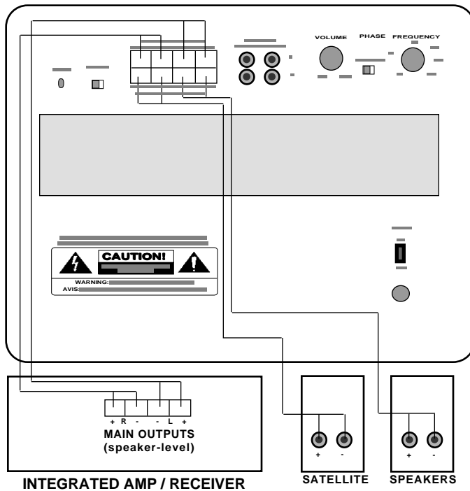
Figure 2: Installation using speaker-level (from amplifier) inputs
